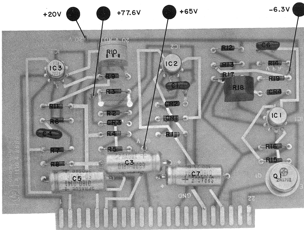
Figure 2. Component Identification, A14 Assembly (Part of Change 2)
