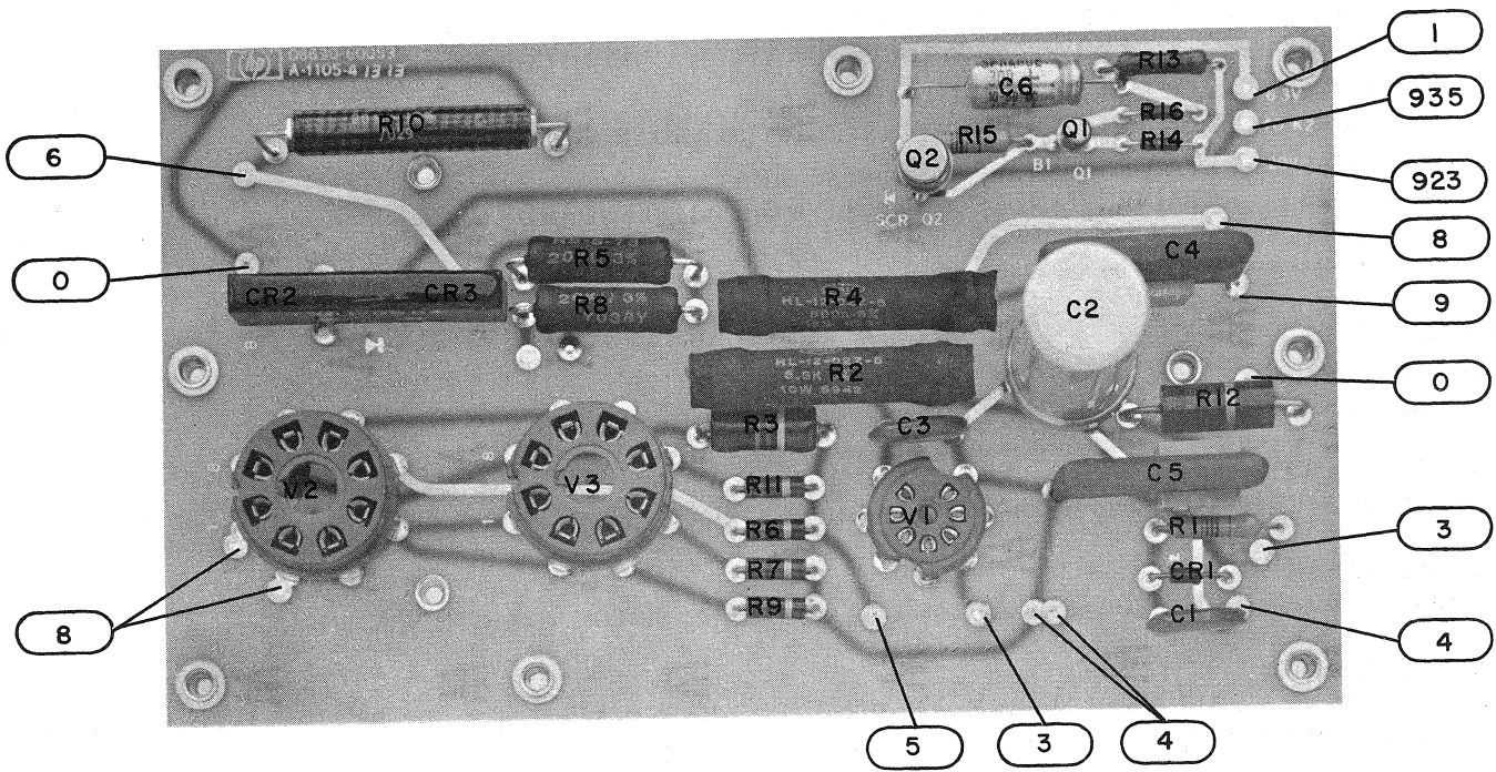
Figure 1. Component Identification, A8 Assembly (Part of Change 1)
